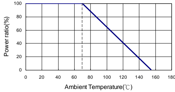
Derating Curve
