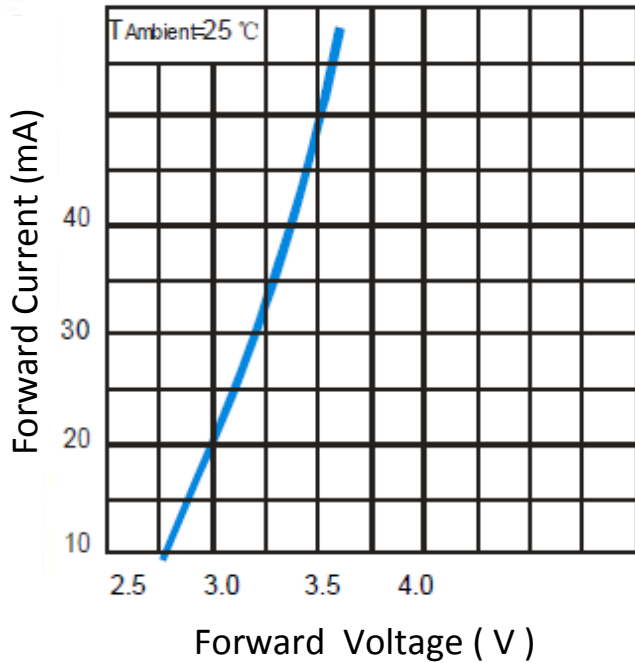
Volt-Ampere Characteristics
