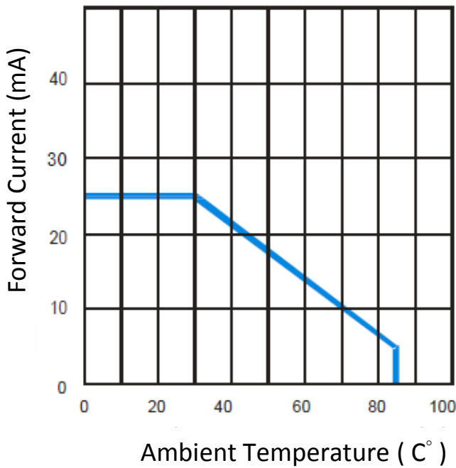
Forward Current Derating
