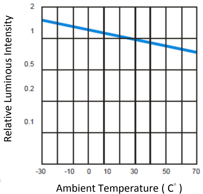
Luminous Intensity VS Ambient
