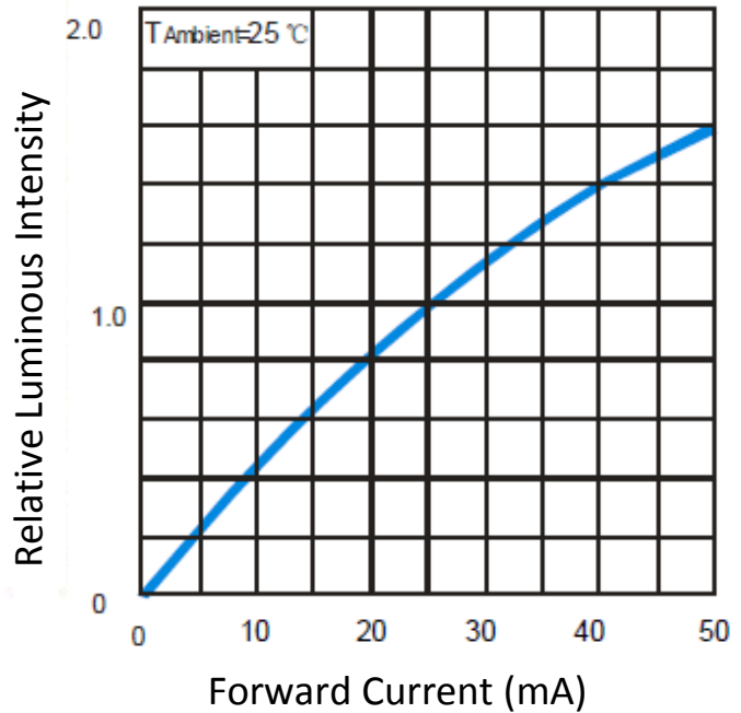
Relative Luminous Intensity VS Forward
